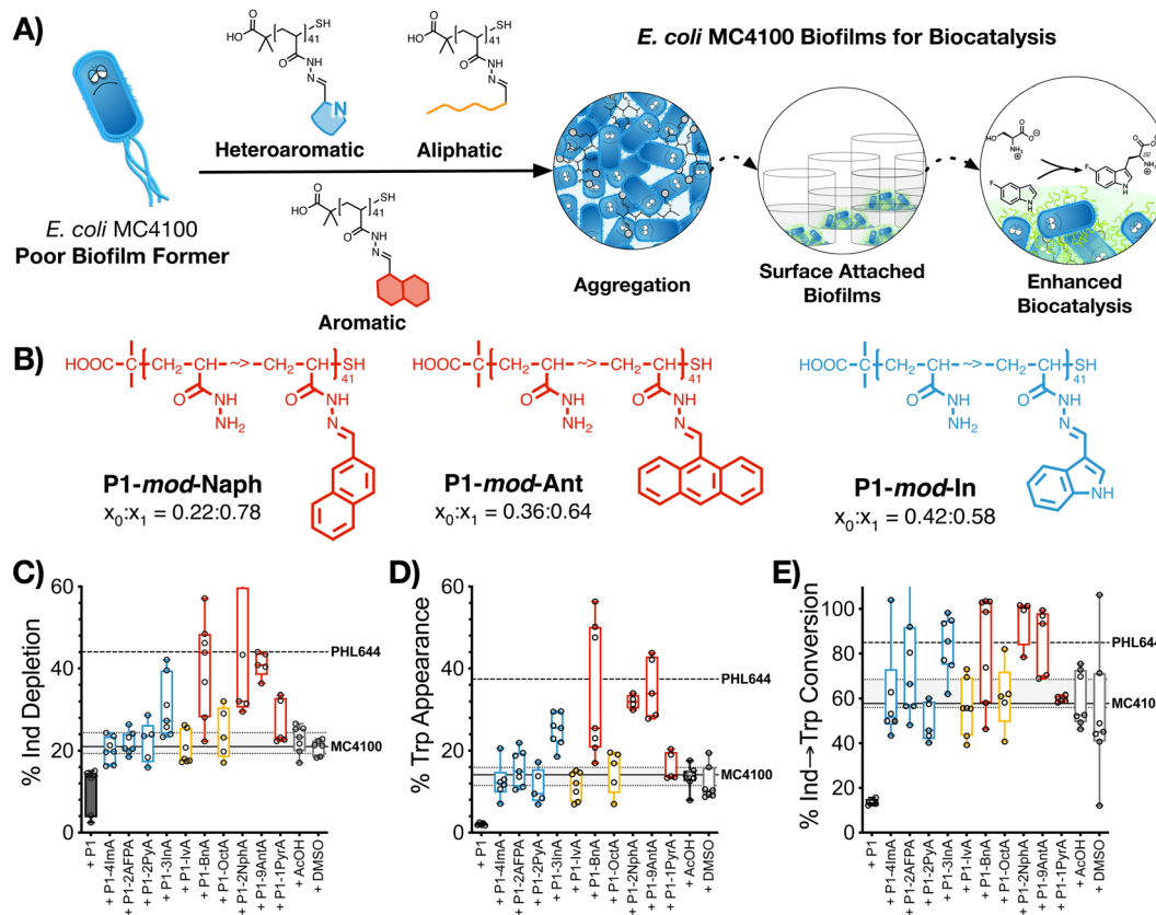
Fig. 4 Biocatalytic activity: (A) schematic representation of polymer-induced biofilms for biocatalysis. (B) Best preforming polymers identified in this assay. (C) Percentage of 5-fluoroindole depletion, (D) 5-fluorotryptophan appearance and (E) conversion of 5-fluoroindole to 5-fluorotryptophan for E. coli MC4100 pSTB7 cultures following 48 h of incubation in 100 mM phosphate buffer at pH 7 in the presence of 0.05 mg mL -1 of P1 (black solid box) and functional polymers P1-mod-aldehyde (hollow boxes), followed by incubation with reaction buffer for another 24 h. Median is shown as a line. Box extends from 25th to 75th percentile while whiskers go from minimum to maximum value. Values for E. coli MC4100 (solid line with 25th to 75th percentile) and E. coli PHL644 cultures (dashed line) incubated in the absence of polymers shown for comparison.
