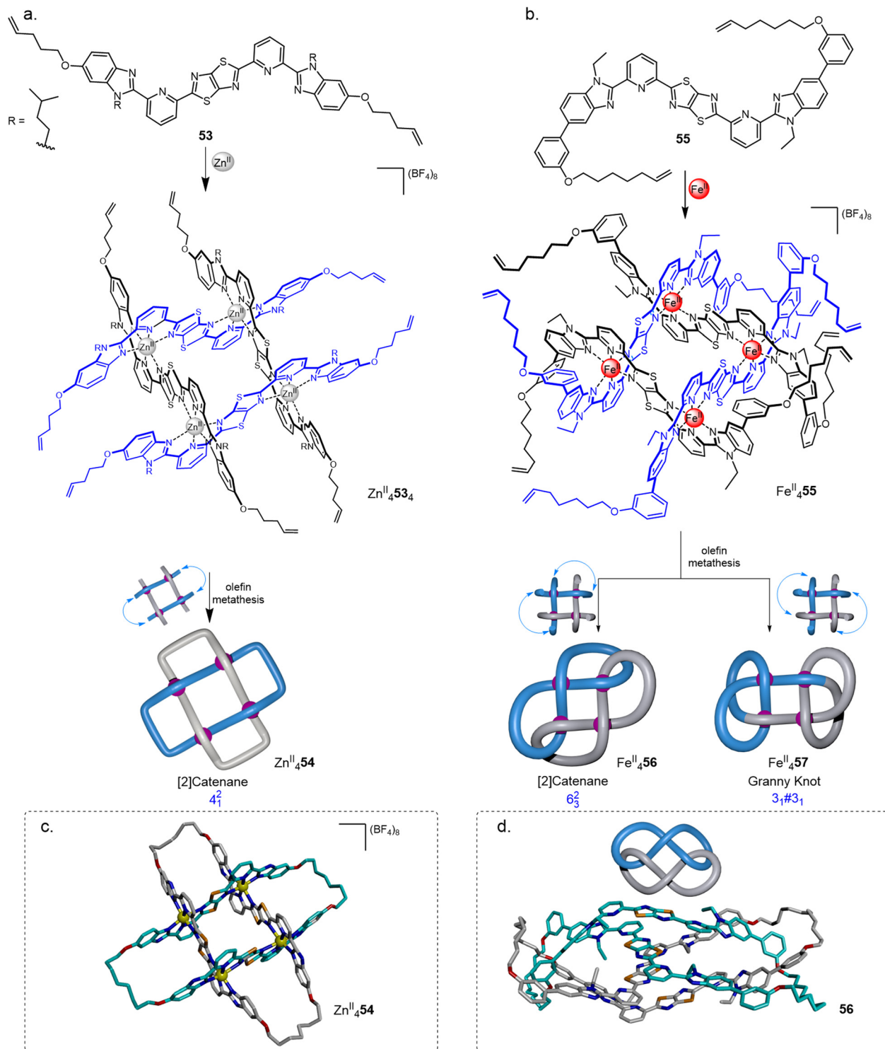
Fig. 20 Synthesis of 2 \times 2 interwoven molecular grids and their closures by olefin metathesis to generate (a) Solomon link 54 , 14 or (b) 6_3^2 link 56 and granny knot 57 , 15 X-ray crystal structures of (c) \text{Zn}^{\text{II}}_4 54 and (d) demetallated link 56 .
