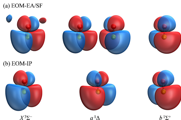
Fig. 3 The Dyson orbitals corresponding to detachment transitions from \text{SO}^- ( X^3\Pi ) to the X^3\Sigma^- , a^1\Delta , and b^1\Sigma^+ electronic states of neutral SO. The orbitals shown in (a) were calculated using transitions from EOM-EA-CCSD to EOM-SF-CCSD states, each starting from the common triplet-state reference, [\dots]^{22}(\pi\alpha)^1(\pi'\alpha')^1 , where \pi and \pi' are the canonical HOMOs of \text{SO}(X^3\Sigma^-) and [\dots]^{22} is the closed-shell configuration comprised of 22 electrons. The orbitals in (b) were obtained using EOM-IP-CCSD, starting from the [\dots]^{22}(\pi\alpha)^1(\pi\beta)^1(\pi'\alpha')^1 anion reference. The two orbitals for the a^1\Delta state shown in (a) describe the degenerate [\dots]^{22}(\pi\alpha)^1(\pi\beta)^1(\pi'\alpha')^1 \rightarrow [\dots]^{22}(\pi\alpha)^1(\pi\beta)^1 and [\dots]^{22}(\pi\alpha)^1(\pi'\alpha')^1(\pi'\beta')^1 \rightarrow [\dots]^{22}(\pi'\alpha')^1(\pi'\beta')^1 transitions accessible from the triplet reference. Only the former is accessible from the anion reference and hence only one a^1\Delta orbital is shown in (b). The calculations were done using the aug-cc-pVTZ+5s5p5d5f basis set at the CCSD(T)/aug-cc-pVTZ optimized geometry of the anion. Isosurface values 0.02.
