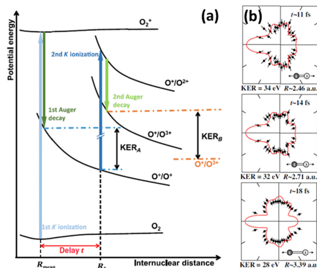
Fig. 5 Schematic of the PAP two-photon K-shell ionization of \text{O}_2 leading to the (\text{O}^+ + \text{O}^{3+}) channel 377 based on typical potential energy curves, featuring the internuclear distance R_2 and delay t for the second photon absorption (a); measured (dots) and computed (red line) PA-MFPADs for three KERs assigned to (R,t) parameters, assuming a second photon absorption by the K orbital of the right-hand O ion (labeled "3" in the inset) (b). Figure adapted from Fig. 2 and Fig. 6 of ref. 377 with permission from Physical Review X under Creative Commons Attribution 4.0 International license ( http://creativecommons.org/licenses/by/4.0/ ).
