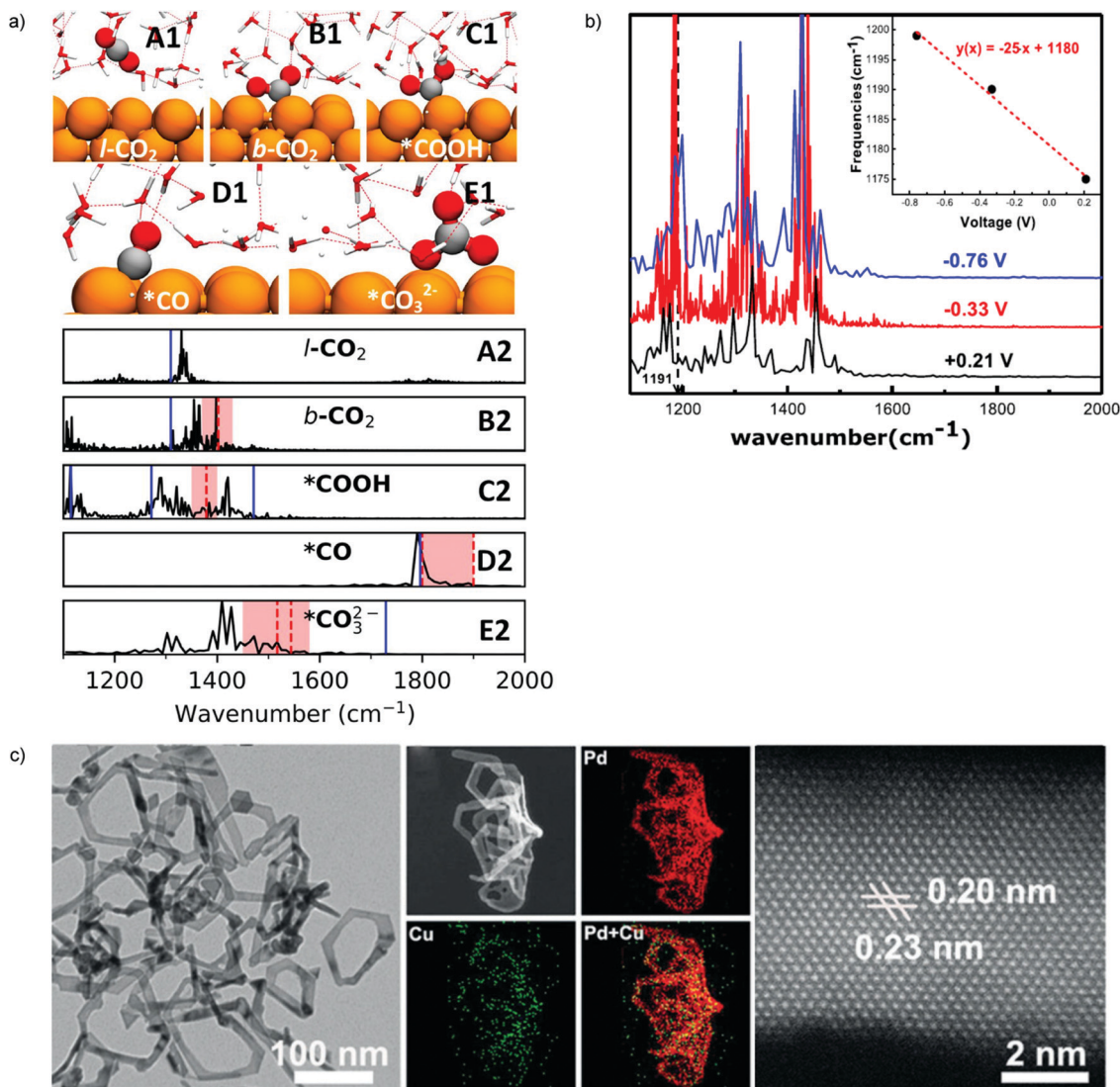
Fig. 9 (a) Snapshots of the structures and v-DoS \text{CO}_2 ( l\text{-CO}_2 ), chemisorbed \text{CO}_2 ( b\text{-CO}_2 ), \text{*COOH} , \text{*CO} , and \text{*CO}_3^{2-} from o-QM-MD simulations and 2PT analysis. The color codes are Cu in orange, O in red, C in silver, and H in white. The hydrogen bonds are shown as dashed red lines. In bottom part, v-DoS from o-QM-MD is shown as a solid black line, the experimental frequencies are shown as a red dashed line, and the vibrational frequencies from v-QM optimization are shown as solid blue lines for comparison. ( l\text{-CO}_2 and b\text{-CO}_2 are the same from v-QM, because b\text{-CO}_2 is unstable in vacuum and automatically converts to l\text{-CO}_2 after optimization.) (b) The simulated potential-dependent v-DoS of \text{*HOC-COH} at +0.21 V, -0.33 V, and -0.76 V. Inset shows the blue shift of the 1191\text{ cm}^{-1} peak (a feature of C-O stretch of C-OH) as a function of applied potential. (c) Characterization of Pd/Cu NRs. From left to right: TEM image; HAADF-STEM image and the corresponding STEM-EDX elemental mapping; atomic resolution HAADF-STEM image. (a) and (b) are adapted with permission from ref. 187, (c) is adapted with permission from ref. 181, Copyright 2017 Wiley-VCH Verlag GmbH & Co. KGaA, Weinheim.
