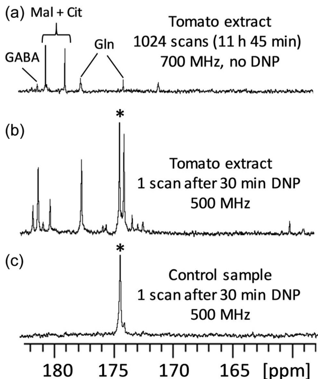
Fig. 5 ^{13}\text{C} NMR spectra (quaternary region) of mature green tomato fruit pericarp extracts. (a) Conventional (non-hyperpolarised) spectrum of 20 mg extract (prepared from 20 mg lyophilized grounded tissue) dissolved in 700 \mu\text{L} \text{D}_2\text{O} , recorded with 1024 scans (11 h 45 min) at 700 MHz with a cryogenic probe. (b) Spectrum of an identical extract recorded with D-DNP combined with CP. The extract was first dissolved in a 200 \mu\text{L} mixture of \text{H}_2\text{O}/\text{D}_2\text{O}/\text{glycerol-}d_8 (2:3:5) doped with 25 mM TEMPOL, then polarized for 30 min at 1.2 K and 6.7 T, and finally dissolved with 5 mL of hot \text{D}_2\text{O} and transferred in about 10 seconds to a 500 MHz spectrometer equipped with a cryogenic probe. (c) Same as (b), but the tomato extract was replaced by a control sample prepared under strictly identical conditions without any biological material. The hyperpolarized spectra result from the sum of six consecutive acquisitions using 30^\circ pulses spaced by 7.7 s. *Indicates the signal of a ^{13}\text{C} -labeled pyruvate impurity from the D-DNP setting. Cit: citrate; GABA: \gamma -aminobutyrate; Gln: glutamine; Mal: malate. Reproduced from ref. 102 with permission from the Royal Society of Chemistry.
