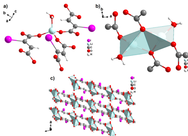
Fig. 42 Crystal structure of [Li(HOOC–CH=CI–COO)(H 2 O)] showing: (a) the coordination sphere of the Li + cation, (b) the dinuclear building unit, and (c) stacked two-dimensional layers. Graphics redrawn from the cif file (CSD-Refcode WAVXEX). 132
