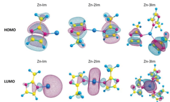
Fig. 4 HOMO and LUMO orbitals of ZIF-8 cluster models with 1, 2 or 3 imidazole rings (Zn-1Im, Zn-2Im, Zn-3Im). Reproduced from ref. 62 with permission from Elsevier, copyright 2021.
