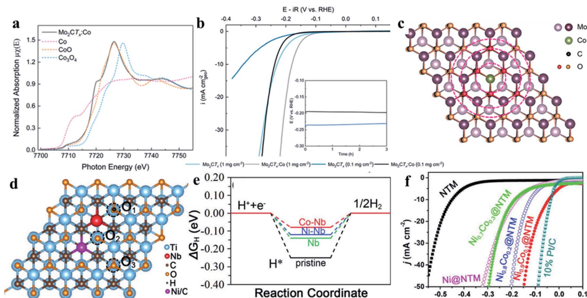
Fig. 10 (a) Comparison of the normalized Co K-edge XANES spectra of \text{Mo}_2\text{CT}_x:\text{Co} with Co, CoO, and \text{Co}_3\text{O}_4 as the references; (b) background-corrected polarization curves recorded for \text{Mo}_2\text{CT}_x:\text{Co} and \text{Mo}_2\text{CT}_x using a scan rate of 10 \text{ mV s}^{-1} , the inset shows chronopotentiometry data for both catalysts at 0.1 \text{ mg cm}^{-2} loading held at 1 \text{ mA cm}^{-2} ; (c) \text{Mo}_2\text{CO}_2:\text{Co} model structure used for DFT calculations, reprinted with permission from ref. 72, Copyright (2019) American Chemical Society for (a)–(c); (d) atomistic configuration of Co/Ni replaced Ti atom on Nb-doped pristine monolayer \text{Ti}_3\text{C}_2\text{O}_2 and the three different \text{H}^* adsorption O sites; (e) Gibbs free energies for \text{H}^* adsorbed at active site on the M-doped \text{Ti}_3\text{C}_2\text{O}_2 monolayer; (f) HER polarization curves of the series NiCo@NTM nanohybrids, Ni@NTM nanohybrid, NTM, and 10% Pt/C in 1 M KOH with a scan rate of 5 \text{ mV s}^{-1} , reprinted with permission from ref. 126, Copyright (2019) Wiley-VCH Verlag GmbH & Co. KGaA, Weinheim for (d)–(f).
