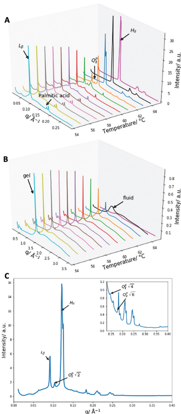
Fig. 6 X-Ray diffraction data of 2 : 1 PA:DPPE-me 2 mixtures (A) SAXS patterns from 54 to 65 °C with an identification of the main liquid-crystalline phase peaks and the excess palmitic acid precipitate. (B) WAXS patterns from 54 to 65 °C with an indication of the gel and fluid phases. (C) The SAXS diffraction pattern at 62 °C, the first peaks of the main liquid crystalline phases and all of the Q_{II}^P phase peaks are identified, and the inserted smaller graph enlarges the peaks in the region from 0.14 to 0.4 Å -1 .
