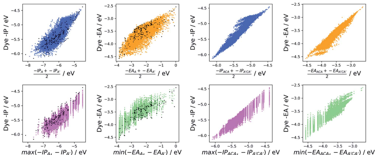
Fig. 7 Property–property relationships between the ACA' dyes and their constituent building blocks as described by the averaging model (top row) and the max/min model (bottom row) using the building block properties (left four panels) and ACA dyes (right four panels) as input. Points for the ACA dyes shown in black.
