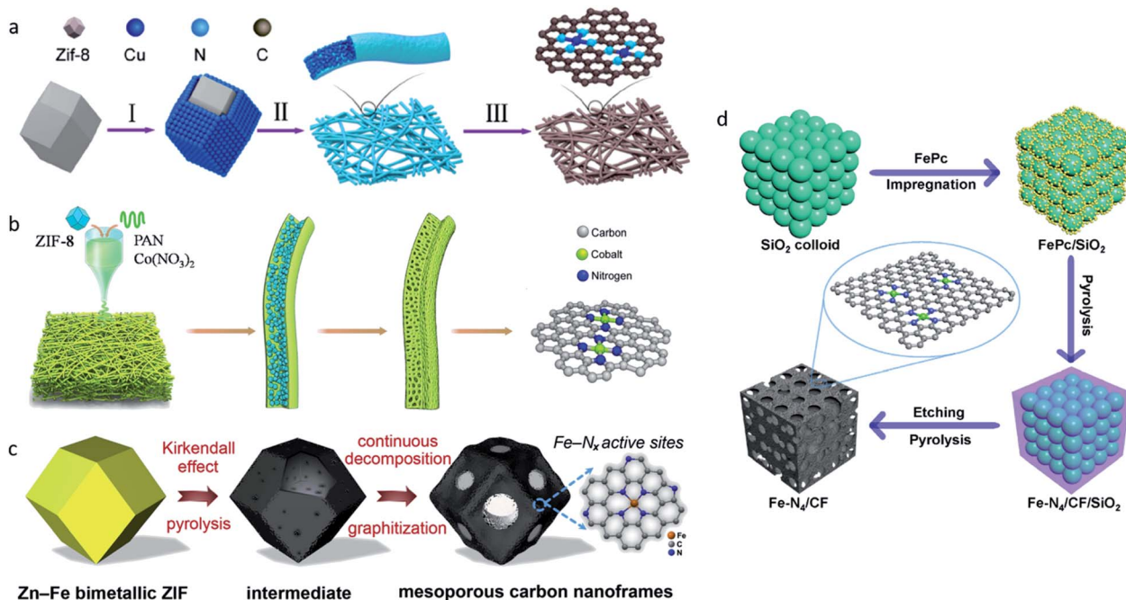
Fig. 8 (a) A schematic illustration of the synthesis of CuSAs/THCF. Reproduced from ref. 98 with permission from American Chemical Society, copyright 2019. (b) A schematic illustration of the synthesis of CoSA/HCNFs. Reproduced from ref. 99 with permission from Elsevier, copyright 2020. (c) A schematic illustration of the synthesis of FeSAs/CNF-900. Reproduced from ref. 100 with permission from Elsevier, copyright 2020. (d) A schematic illustration of the synthesis of Fe–N 4 /CF. Reproduced from ref. 12 with permission from Springer Nature, copyright 2019.
