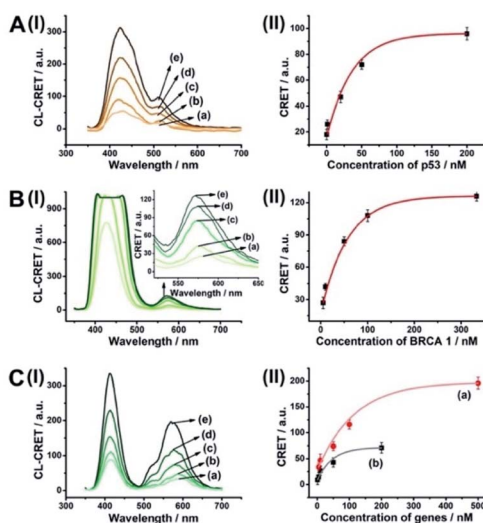
Fig. 9 Multiplexed analysis of the p53 and BRCA1 genes by a mixture consisting of FI-loaded hp9-modified NMOFs and Rh 6G-loaded hp10-modified Rh 6G-loaded NMOFs using the HCR-amplified CRET-induced analysis of the two genes upon (panel A) subjecting the mixture to variable concentrations of p53: (a) 0 nM; (b) 1 nM; (c) 20 nM; (d) 50 nM; (e) 200 nM; (panel B) subjecting the mixture to variable concentrations of BRCA1: (a) 0 nM; (b) 5 nM; (c) 50 nM; (d) 100 nM; (e) 333 nM; and (panel C) subjecting the mixture to variable concentrations of p53: (a) 0 nM; (b) 1 nM; (c) 10 nM; (d) 50 nM; (e) 200 nM (curve (b) in panel II), and to variable concentrations of BRCA1: (a) 0 nM; (b) 5 nM; (c) 50 nM; (d) 100 nM; (e) 500 nM (curve (a) in panel II). Error bars derived from N = 3 experiments.
