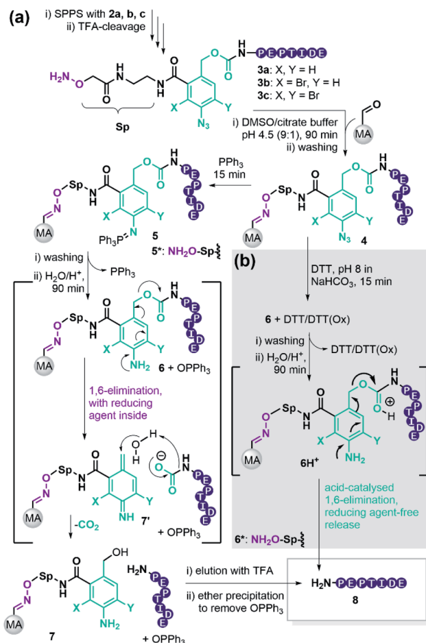
Scheme 2 (a) Application of reductively cleavable linker 2a, b, c in c8r purification of peptides with PPh 3 as reductive stimulus; MA: modified agarose beads, GdmCl: Guanidinium chloride. (b) Usage of dithiothreitol (DTT) as reductive stimulus, *: linker-modified peptide in solution.
