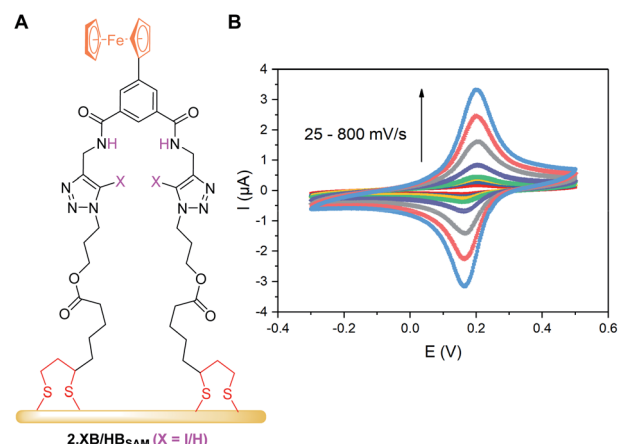
Fig. 4 (A) Schematic representation of 2.XB/HB SAM on a gold electrode. (B) CVs at varying scan rate of 2.HB SAM in ACN, 100 mM TBAClO 4 . The associated anodic and cathodic peak currents as a function of the square-root of the scan rate are shown in Fig. S25.†
