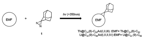
Scheme 1 Reaction of 1 with \text{Th}@C_{3v}(8)\text{-C}_{82} or \text{U}@C_{2v}(9)\text{-C}_{82} .
