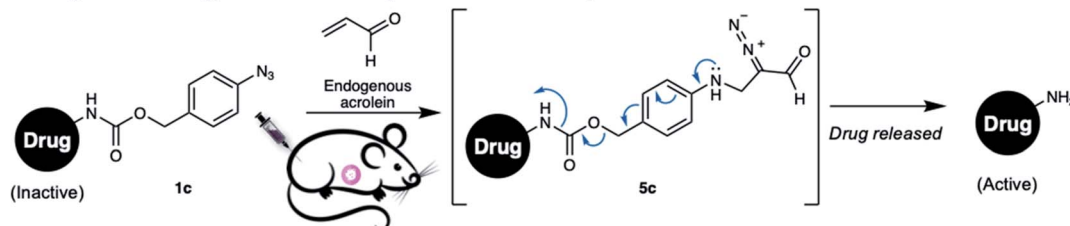
(c) This work: Drug release strategy based on the endogenous acrolein-azide cycloaddition
