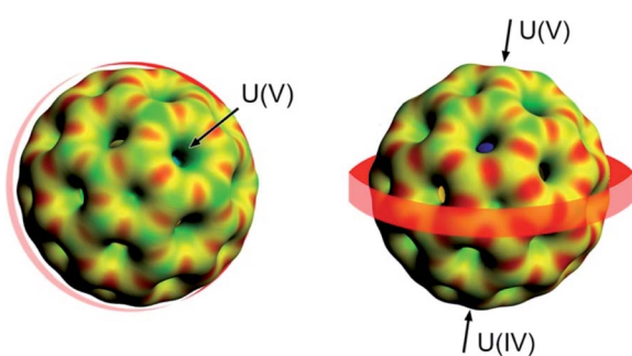
Fig. 5 Two views of the molecular electrostatic potential (MEP) for U_2N@C_{80} . Red identifies regions in which the MEP is low (nucleophilic regions) and green identifies regions where the MEP is high (electrophilic regions). The equatorial region between the two U atoms, found to be the most electrophilic part of the cage, is highlighted with a red belt.
