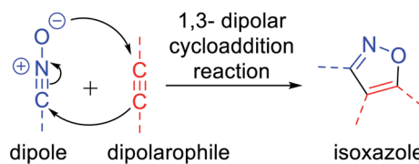
Fig. 2 Mechanism of 1,3-dipolar cycloaddition reaction.
