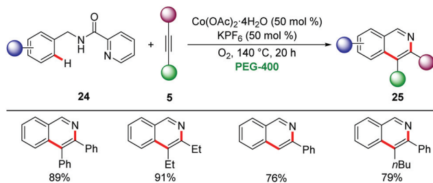
Scheme 7 Cobalt-catalyzed synthesis of isoquinolines 25 in PEG-400.
