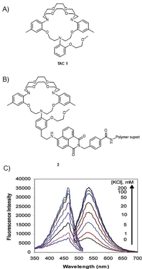
Fig. 1 (A) Ttriazacryptand[2,2,3]-1-(2-methoxyethoxy) benzene (TAC). (B) He's design for an optical sensor. (C) Excitation and emission spectra of a sensor disk exposed to different potassium chloride solutions in TRIS-HEPES buffer at pH 7.40 (left, excitation spectra, fixed emission at 540 nm; right, emission spectra, fixed excitation at 470 nm. Reproduced with permission ref. 32, copyright American Chemical Society.
