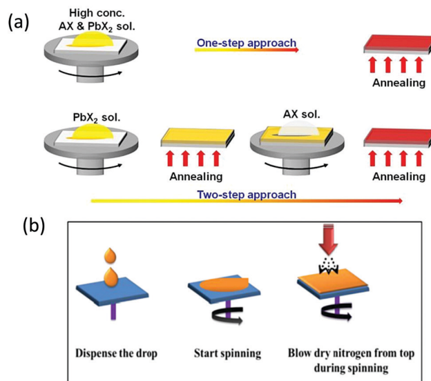
Fig. 6 Representation of one-step and two-step strategies for the preparation of perovskite films. AX and PbX 2 symbolize CsBr and PbBr 2 , respectively. Reprinted with permission ref. 106. Copyright 2019, The Royal Society of Chemistry. (b) N 2 gas flow-assisted method for the fabrication of pinhole-free CsPbBr 3 thin films. Reprinted from ref. 119. Copyright 2020, Gupta, Kulbak, and Cahen.
