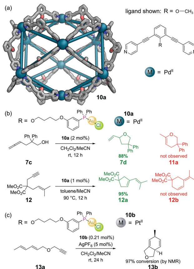
Fig. 12 Reek and co-workers' covalently-tethered phosphine-gold complexes for catalysis. (a) The outer framework of the M 12 L 24 nanosphere 6 solved by SCXRD, with the inner groups and hydrogen atoms omitted for clarity. Colours: C grey, N blue, O red, Pd dark teal (shown as spheres); (b) selectivity in cyclisations catalysed by Pd nanospheres 10a ; (c) the use of Pt nanospheres 10b to accomplish more challenging cyclisations.
