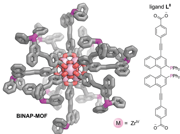
Fig. 11 The Zr 6 O 4 (OH) 4 (O 2 CR) 12 SBUs bound by 12 L B bridging ligands which bridge adjacent clusters to form BINAP-MOF . Post-metalation with [Rh(nbd) 2 ](BF 4 ) yields BINAP-MOF-Rh , which acts as a catalyst for the conjugate addition of arylboronic acids to 2-cyclohexanone. 50 Hydrogen atoms omitted for clarity. Colours: C grey, O red, P magenta, Zr light pink (shown as spheres).
