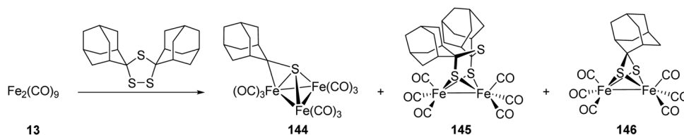
Fig. 42 Synthetic pathways to novel sdt complexes from Fe 2 (CO) 9 .
