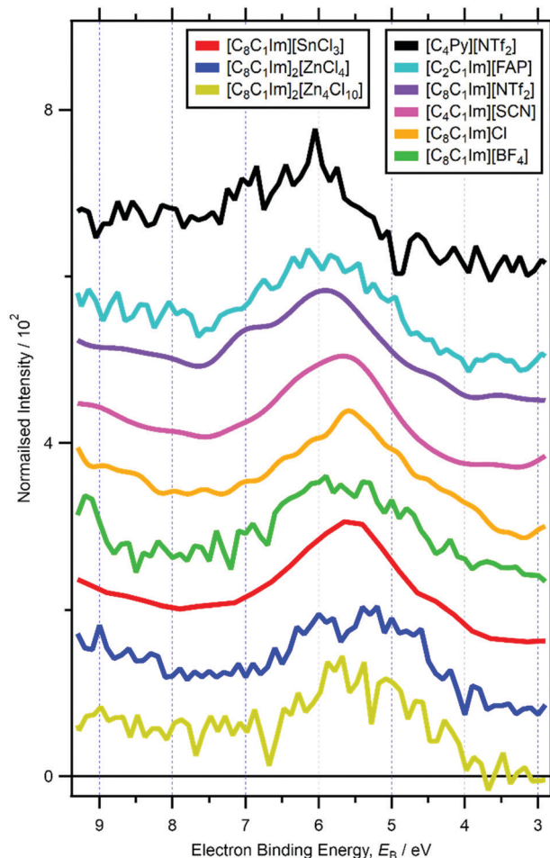
Fig. 4 Subtracted RXP spectra for N_{\text{cation}} for nine ionic liquids ( h\nu \sim 402 eV). These RXPS traces were produced by subtraction of resonant XP spectrum minus non-resonant XP spectrum using the procedure outlined in ref. 48. All electron spectra were charge referenced using methods outlined in Section 2.4.
