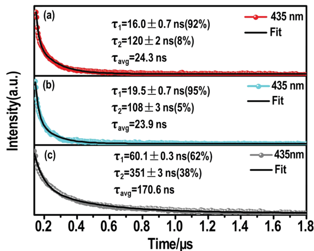
Fig. 4 Nanosecond time-resolve emission (ns-TE) decays and fittings of the (a) ( S -β-MPEA) 2 PbBr 4 , (b) ( R -β-MPEA) 2 PbBr 4 , and (c) (( rac )-MPEA) 2 PbBr 4 emission at 435 nm.
