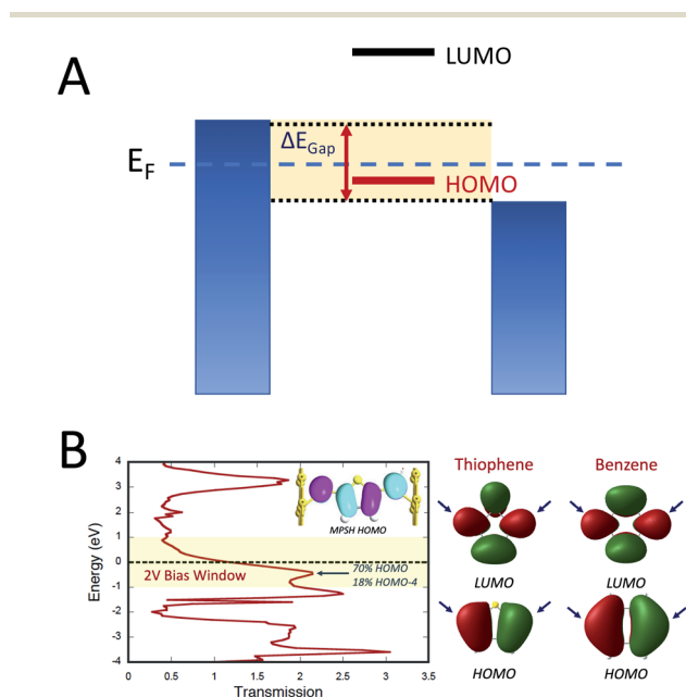
Fig. 5 (A) Illustration of the HOMO conductance mechanism. The biased electrodes (blue) are filled to the chemical potential of the electrodes and the variable bias window ( \Delta E_{\text{Gap}} = V_{\text{bias}} ) is highlighted in yellow. Only the HOMO is dominant in the bias window and therefore it maximally contributes to g_{mb} . The LUMO is at higher energy and lies outside of the bias window. As such, it does not contribute to g_{mb} . (B) Left: Computed zero-bias energy vs. transmission plot for S-Th-S connected to Au electrodes. A 2 V bias window is depicted in yellow and the Fermi energy is shown as a dashed line. Inset: Molecular projected self-consistent Hamiltonian (MPSH) state that dominantly contributes to g_{mb} , which is primarily comprised of the Th HOMO. Right: HOMO and LUMO of Th and Ph. Bridge carbon atoms of contact are indicated by blue arrows.
