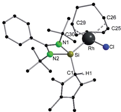
Fig. 6 Solid state structure of compound 6 . Hydrogen atoms are omitted for clarity (except H1). Selected bond lengths [Å] and angles [°]: Rh–Si 2.2947(5); Rh–Cl 2.3785(5); Rh–C25 2.280(2); Rh–C26 2.272(2); Rh–C29 2.094(2); Rh–C30 2.108(2); Si–N1 1.8540(14); Si–N2 1.8443(14); Si–C1 1.911(2); N1–C10 1.336(2); N2–C10 1.339(2); C1–C2 1.514(3); C1–C5 1.501(3); C2–C3 1.343(3); C3–C4 1.468(4); C4–C5 1.339(4); N1–C10–N2 106.92(14); Si–Rh–Cl 87.98(2); C25–Rh–C26 34.68(8); C29–Rh–C30 38.95(7); N1–Si–Rh 112.51(5); N1–Si–C1 108.93(7); N2–Si–Rh 123.17(5); N2–Si–C1 107.78(7); C1–Si–Rh 121.77(6).
