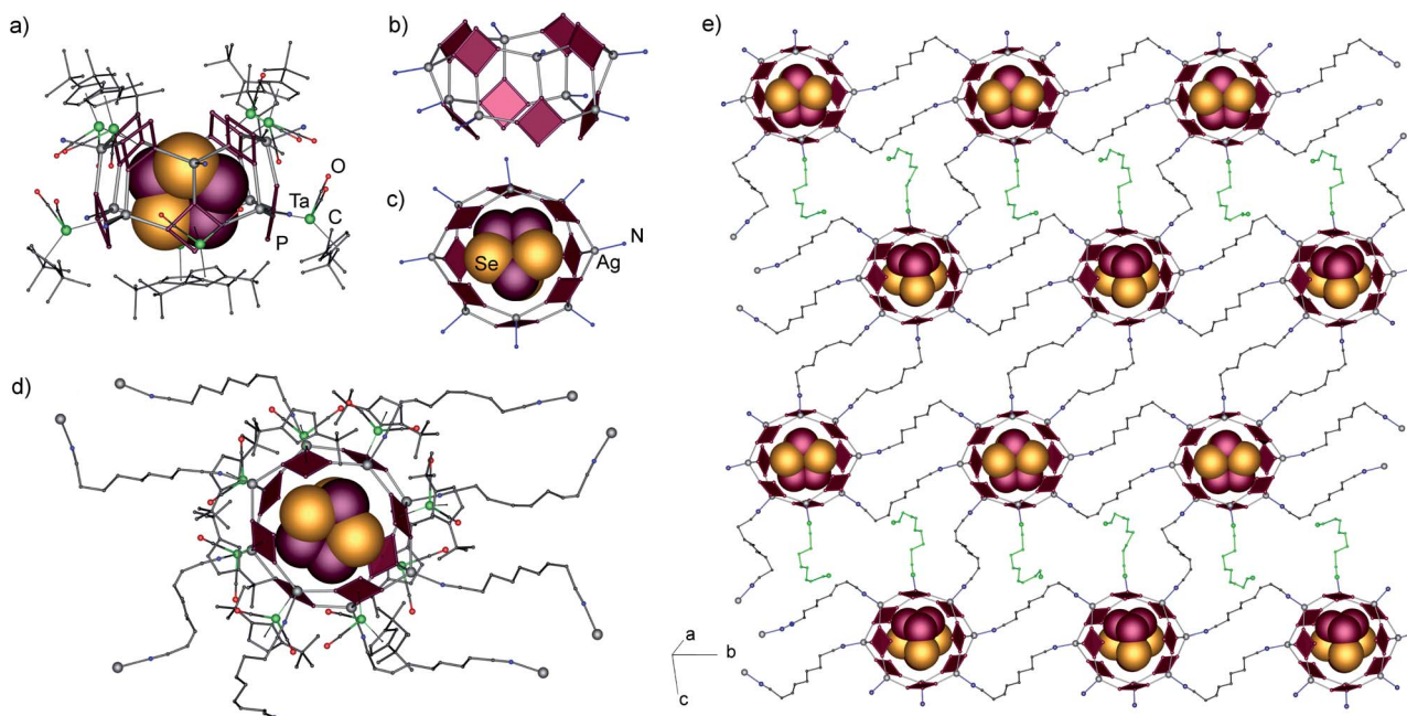
Fig. 4 (a) Supramolecular node, (b) its 40-vertex inorganic core (c) containing a \text{P}_4\text{Se}_3 guest molecule, (d) node with outgoing linkers, (e) 2D network of interconnected nodes in 7 . The guest is depicted in the space-filling model. Non-coordinating linker units are highlighted in green. \{\text{Cp}''\text{Ta}(\text{CO})_2\} fragments and counter-anions are omitted for clarity.
