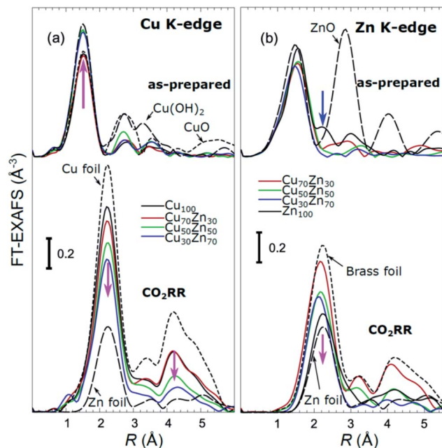
Fig. 4 Cu K-edge (a) and Zn K-edge (b) Fourier-transformed (FT) EXAFS spectra or CuZn NPs with different composition. Spectra for as-prepared samples and for samples in final state after 1–7 hours under \text{CO}_2\text{RR} conditions are shown together with those for reference materials (ZnO, CuO, \text{Cu}(\text{OH})_2 , Zn foil, Cu foil, CuZn brass foil (Cu to Zn ratio 7 : 3)). The spectra are shifted vertically for clarity. Magenta arrows emphasize the changes in the spectra with increasing Zn content. Note that the spectra shown are “phase-uncorrected”, thus the positions of the FT-EXAFS peaks do not correspond to the true positions of the RDF peaks.
