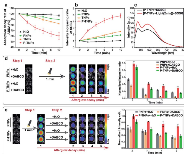
Fig. 3 (a) Normalized absorption decay rate of ABDA (20 μM, final concentration) at 375 nm and (b) normalized fluorescence increase rate of SOSG (2.4 μM, final concentration) at 528 nm in the presence of H 2 O, PNP, TNP and P-TNP solutions upon white light irradiation every 2 min. (c) Fluorescence spectra of SOSG in P-TNP solution and that added after P-TNP irradiation for 2 min. (d) Afterglow luminescence images and quantitative afterglow intensity of PNPs and P-TNPs with pre-added DABCO (250 mM, final concentration) and H 2 O, respectively, obtained after irradiation for 1 min. (e) Afterglow luminescence images and quantitative afterglow intensity of PNPs and P-TNPs irradiated for 1 min, and then addition of DABCO (250 mM, final concentration) and H 2 O, respectively. All the mentioned white light source is a white LED lamp (2000 lm). The error bars represent the s.d. ( n = 3).
