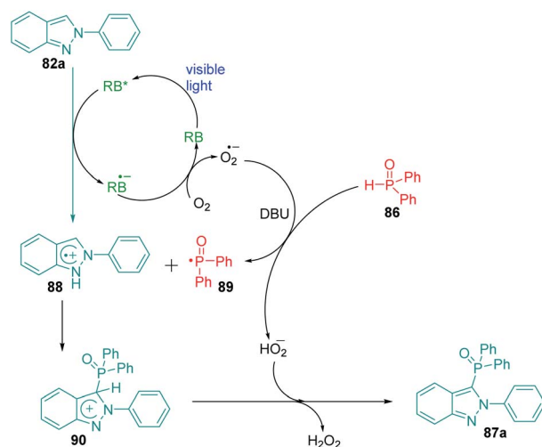
Scheme 26 Rose Bengal catalyzed phosphorylation of indazole.
