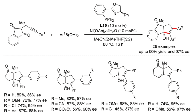
Scheme 30 Ni-Catalyzed enantioselective anti -arylation cyclization of alkynyl electrophiles with organoboronic acids.
