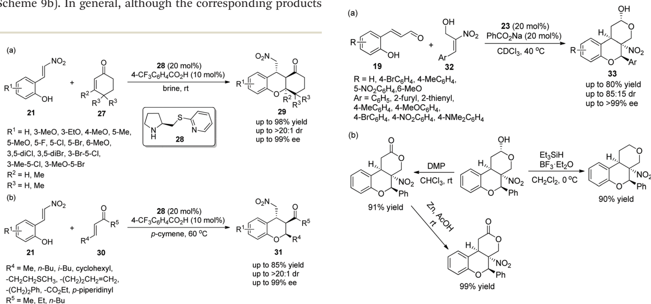
Scheme 10 Oxa-Michael/Michael/nucleophilic ring-closing cascade reaction for the synthesis of chromans and the derivatizations of chiral chroman.
