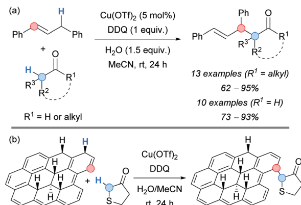
Scheme 50 DDQ-promoted Cu-catalyzed CDC between (a) 1,3-diphenylpropene and aldehydes or ketones or between (b) hydrogenated graphene and tetrahydrothiophen-3-one.
