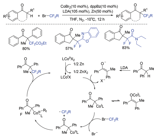
Scheme 104 The cobalt-catalyzed difluoroalkylation of tertiary aryl ketones.
