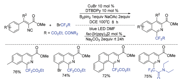
Scheme 109 The Cu/B_2pin_2 -promoted cascade cyclization of vinyl isocyanides.
