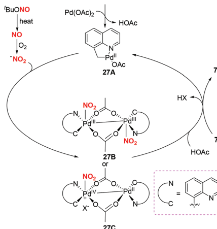
Scheme 27 Palladium-catalyzed sp 3 C–H nitration of 8-methylquinolines.
