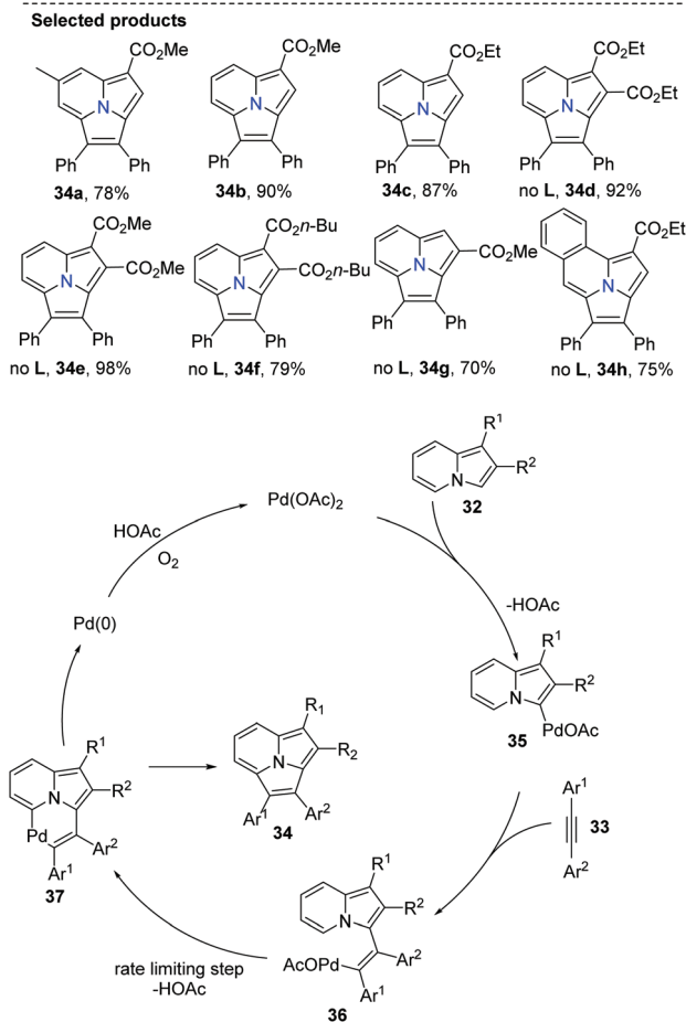
Scheme 5 Dual C-H activation and a plausible mechanism.
