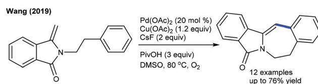
Scheme 90 Direct intramolecular arylation of enamide by C-H activation.
