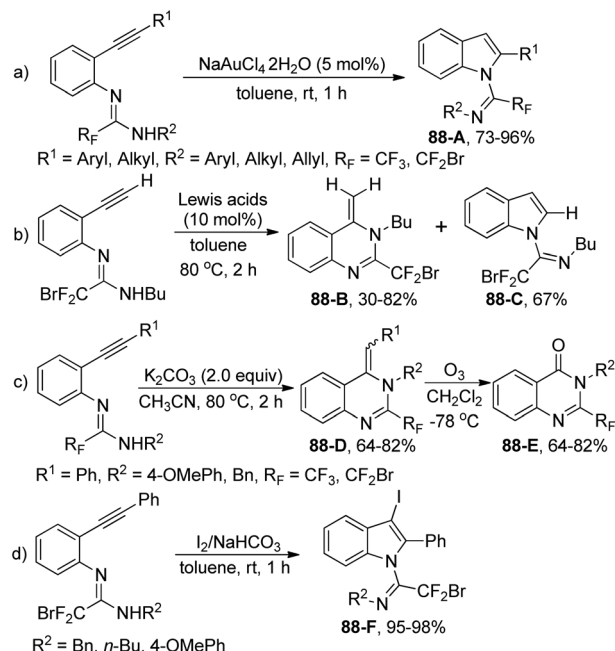
Scheme 88 Intramolecular hydroamination of fluorinated N -( ortho -alkynylaryl)amidines.
