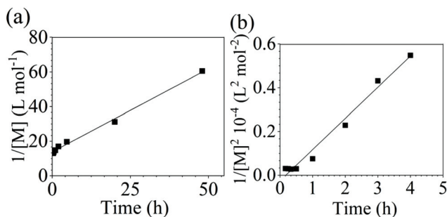
Fig. 4 Linearized kinetic plots of: (a) second-order reaction for the polycondensation of DCDPS/BPA with \text{Na}_2\text{CO}_3 at 160^\circ\text{C} , and (b) third-order reaction for the polycondensation of DFDPS/BPA with \text{Na}_2\text{CO}_3 at 140^\circ\text{C} .
