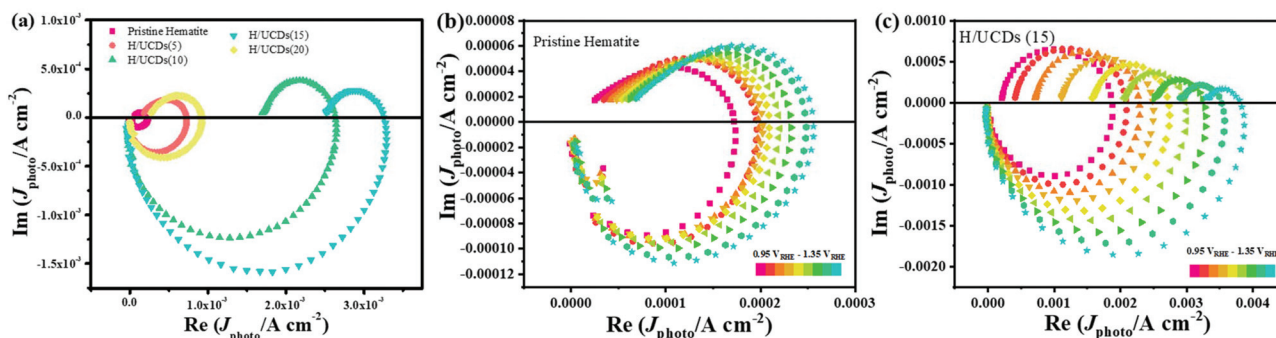
Fig. 6 IMPS plots for (a) pristine hematite and H/UCDs photoelectrodes; (b) pristine hematite; (c) H/UCDs (15).
