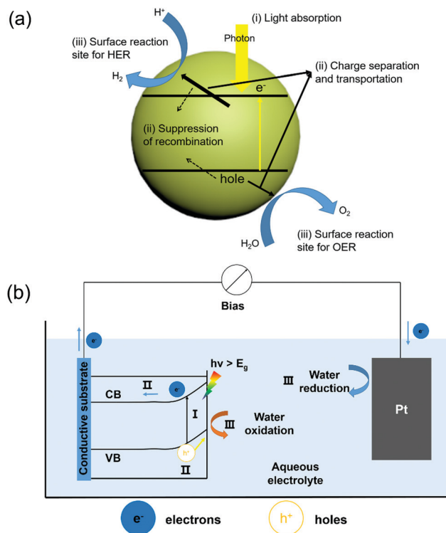
Fig. 1 (a) Schematic of the main process of PC water splitting in a simple photocatalytic semiconductor; (b) diagram of a typical PEC water splitting system with an n-type semiconductor as the photoanode and Pt as the counter electrode, both immersed in an aqueous electrolyte. In the picture, process I refers to photon absorption and the resulting excitation of an electron from the VB to CB, leaving a hole at the VB. Process II refers to the separation and transportation of photogenerated electron and hole pairs. Process III refers to the surface redox reactions, where water oxidation occurs at the semiconductor surface and the reduction reaction occurs at the Pt surface.
