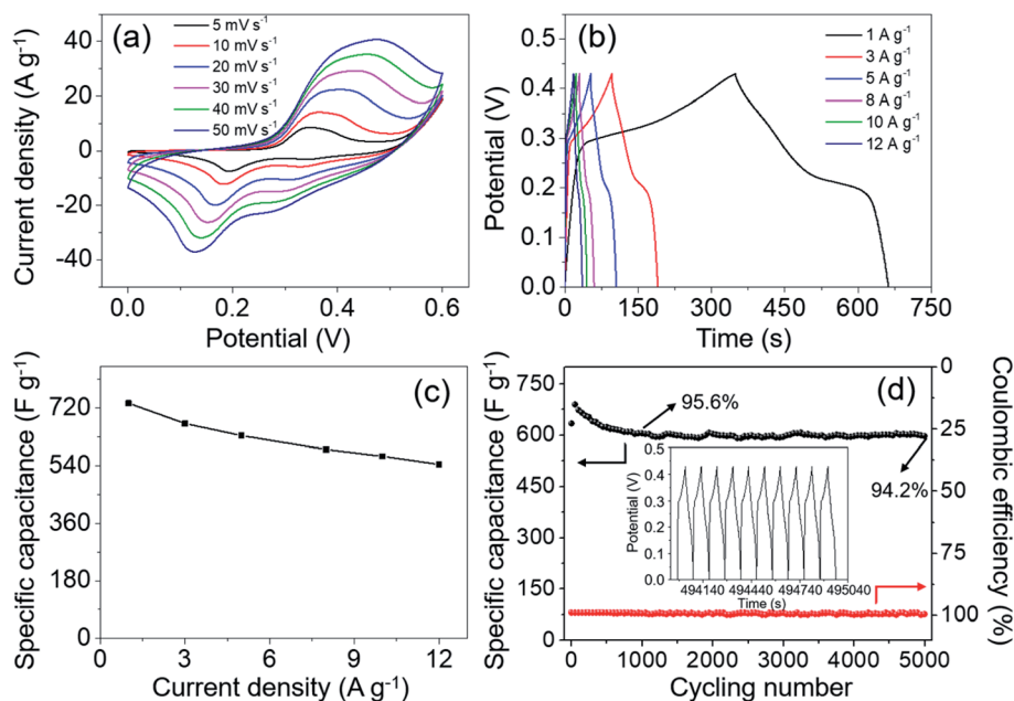
Fig. 8 Electrochemical tests of the MgCo 2 O 4 -NFs-modified electrode in 2 M KOH solution: (a) CV curves obtained at scan rates from 5 to 50 mV s -1 , (b) GCD curves measured at different current densities from 1 to 12 A g -1 , (c) specific capacitance at different current densities, and (d) cycling performance and coulombic efficiency at 5 A g -1 for 5000 cycles with the inset showing the last 10 cycles.
