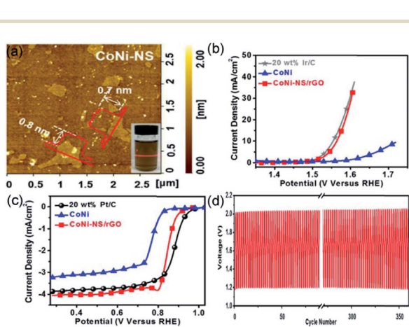
Fig. 7 (a) AFM image of CoNi-NS and photograph of CoNi-NS suspension. Polarization curves of CoNi-NS/rGO, CoNi, and commercial catalysts for (b) OER and (c) ORR. (d) Charge and discharge cycling curves of CoNi-NS/rGO at 10 mA cm -2 . Reproduced from ref. 82. Copyright 2019, Elsevier.
