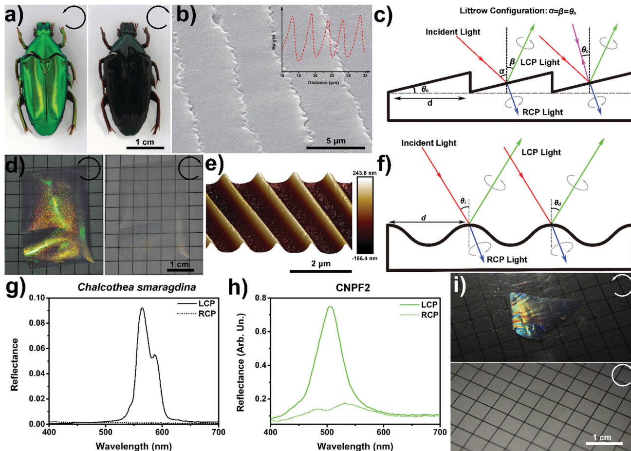
Fig. 5 (a) Photographs of the beetle Chalcothoa smaragdina captured in a LCP (left) and a RCP (right) filter, respectively. (b) SEM image of the periodic surface structure for the beetle. The inset represents the AFM surface profile of the beetle surface, which reveals a blazed grating surface topography. (c) Schematic representation of the polarization-selective surface blazed grating for the beetle exocuticle in which the diffracted LCP light generates constructive interference, whereas for the Littrow configuration (purple lines) the incidence angle and diffraction angle are identical, leading to a special specular reflection. (d) Photographs of CNPF2 captured using a LCP (left) and a RCP (right) filter, respectively. (e) Three-dimensional AFM image of CNPF2 that exhibits a smooth sinusoidal surface profile. (f) Schematic description of the chiral nematic ordered holographic surface grating with selective constructive interference for LCP light. (g and h) LCP and RCP reflectance spectra for the beetle of Chalcothoa smaragdina (g) and CNPF2 (h), respectively. (i) Photographs of CNPF1 with strong photonic–photonic coupling captured in a LCP and RCP filter. (a), (b) and (g) were adopted with permission from ref. 11.
