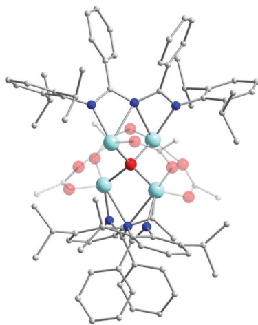
Fig. 6 The molecular structure of the cationic complex 19 . 48a For clarity reasons H-atoms and disorder conformers have been omitted, as well as partial transparency has been employed. Colour code: C: grey, N: blue, O: red \text{Zn}^{\text{II}} : pale blue. Reproduced using reported cif.
