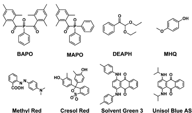
Fig. 4 Chemical structure of the selected photopolymerization initiators (MAPO, BAPO and DEAPH), terminator (MHQ) and dyes.
