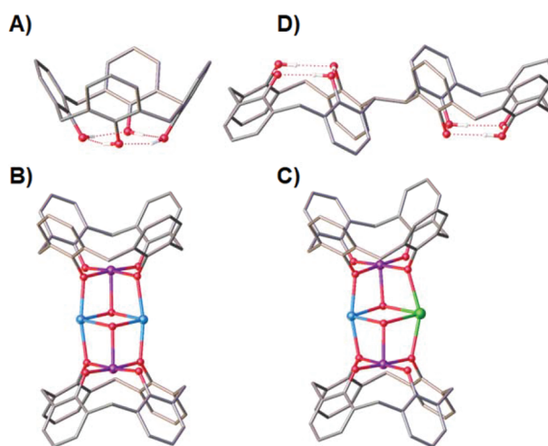
Fig. 1 Single crystal X-ray structures of TBC[4] (A), 1 (B), 2 (C), H 3 L (D). Colour code C – grey, O – red, Mn II – pale blue, Mn III – purple, Gd III – green, H – white. Hydrogen atoms (except those involved in lower-rim H-bonding in A and D), t Bu groups, ligated solvent molecules and co-crystallised solvent/anions omitted for clarity.
