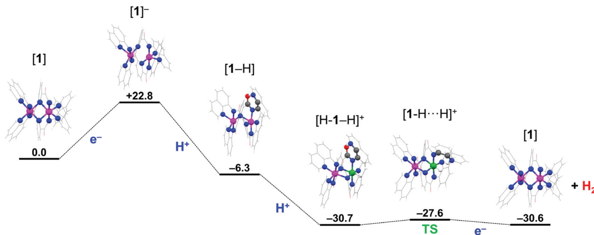
Scheme 3 Proposed pathway of the electrocatalytic reduction of protons to H 2 using 1 as catalyst, showing optimized structures. Color scheme: Co(II), magenta; Co(III), jade; O, red; N, blue; C, pewter; H, white. Relative energies at the B3LYP/ZORA-def2-TZVPP + COSMO level are in kcal mol -1 .
